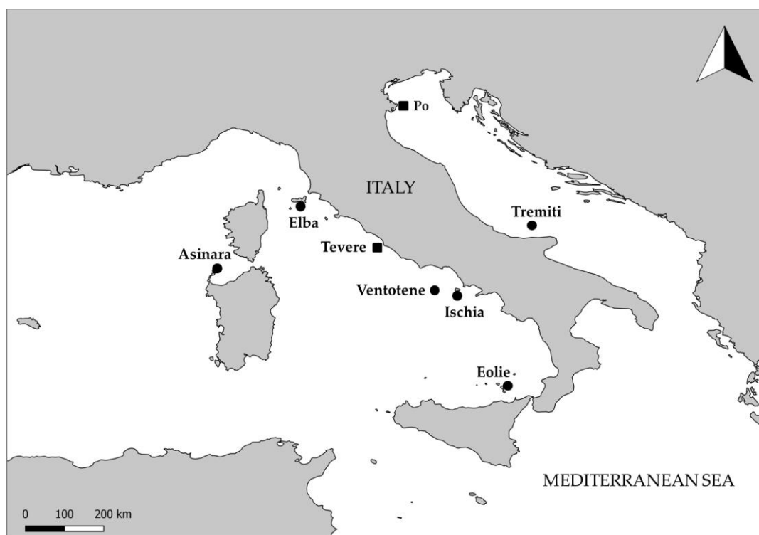
Figure 1. Map of the study area. In each site, 8 replicates (4 mantra trawl (MA) + 4 plankton net (WP2)) were performed, with the exception of the Tevere and Po sites where only MA was employed. The minor islands are shown as circles and the river mouths as squares.
