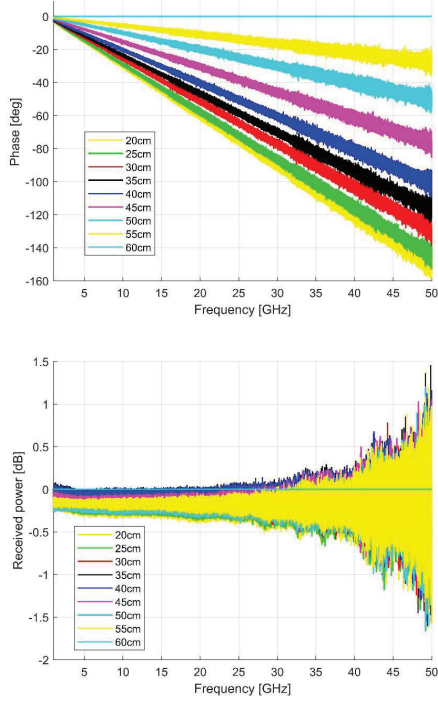
Figure 2. Phase (top) and amplitude (below) response over frequency band with different cable bending diameters.
