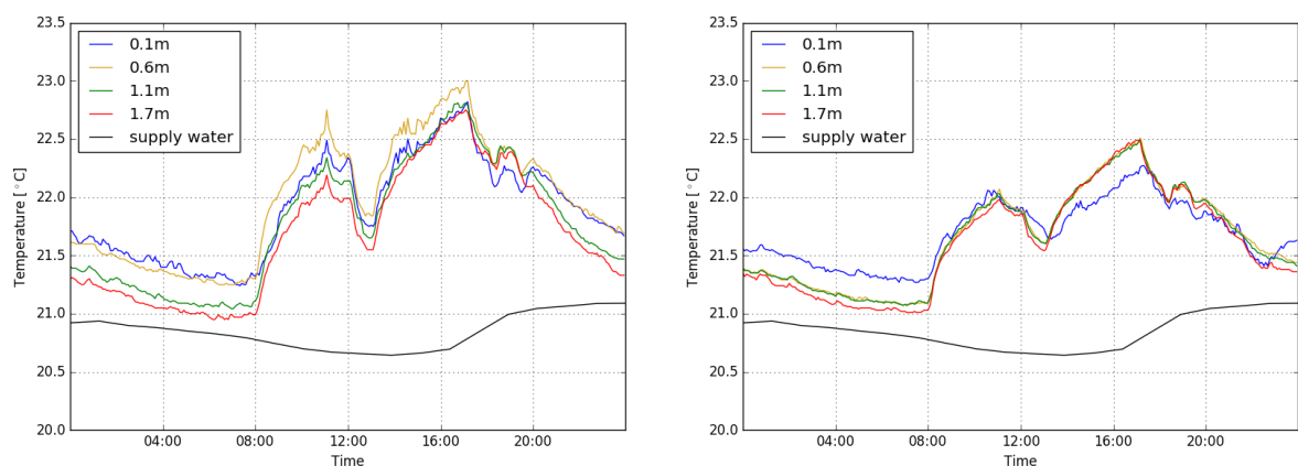
Figure 6 Air temperature profiles for the summer day – 22 th of August: P1 (left) and P2 (right)
