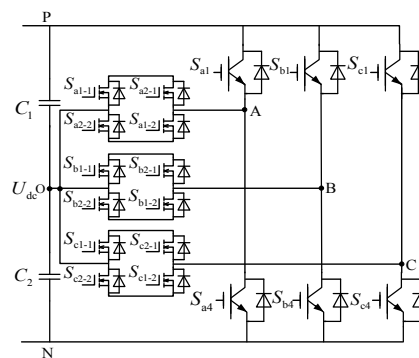
Fig.1 Improved T-type three-level inverter topology
