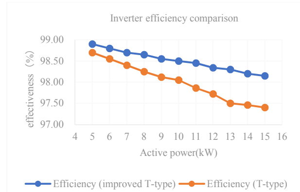
Fig.13 Efficiency comparison between improved T-type three-level inverter and T-type three-level inverter
