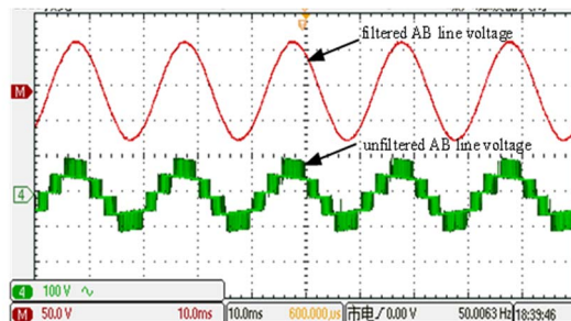
Fig.17 The output AB line voltage experimental waveform
