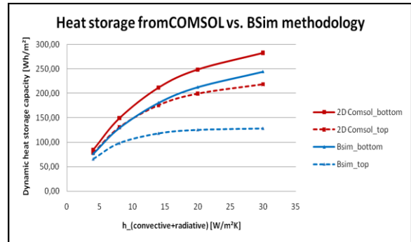
Figure 8 Validation of calculation methodology for heat storage in BSim.
