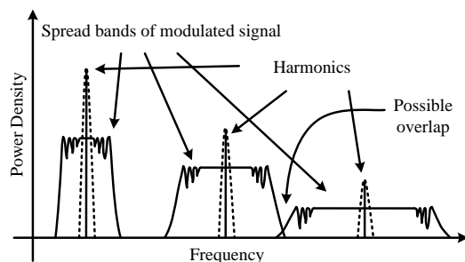
Fig. 2. Spread bands of harmonics in modulated square signals.
