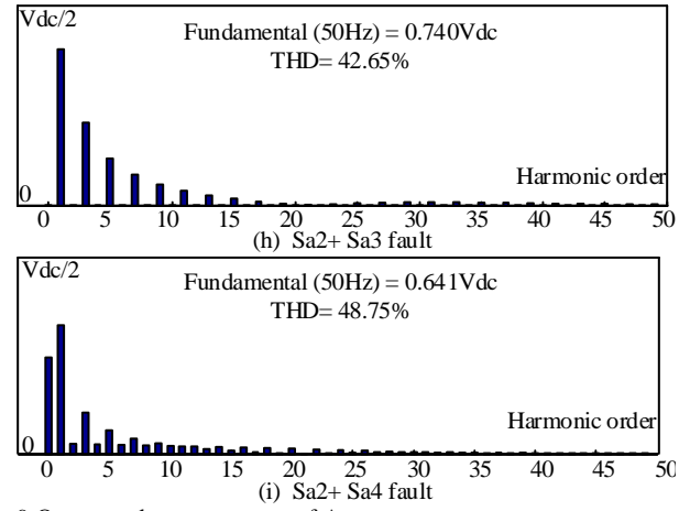
Fig. 9 Output voltage spectrum of Arm a
