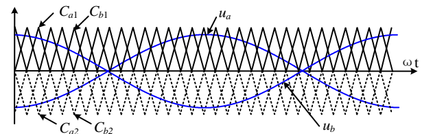
Fig.3 Modulation strategy of single phase 3L-NPC-CI
