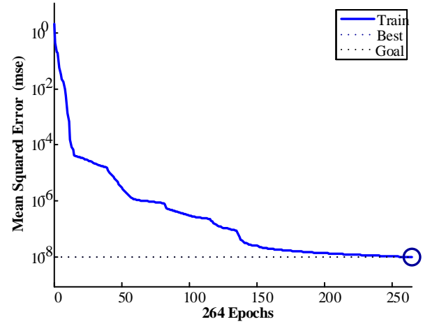
Fig.11 Convergence curve of neural network
