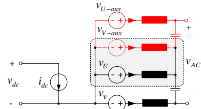
(a) Synthesis topologies based on Full-bridge converters
