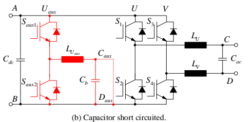
Fig. 7. Two topology examples that do not work following the principle in synthesis procedure.
