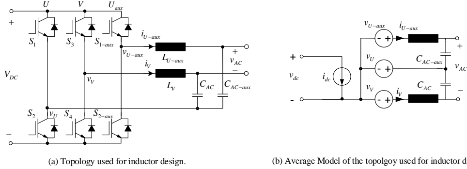
Fig. 13. Three legs single-phase structure used for the inductor design and analysis.
