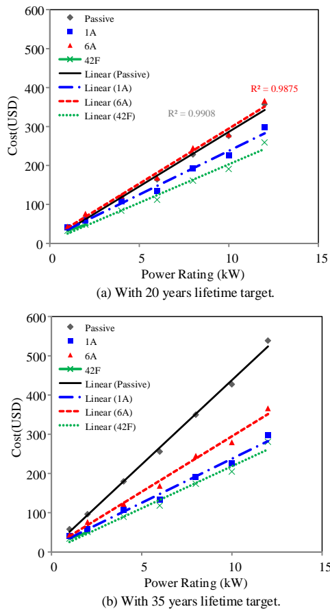
Fig. 21. Cost evaluate results of four cases with 20 and 35 years lifetime target and scalable power rating.
