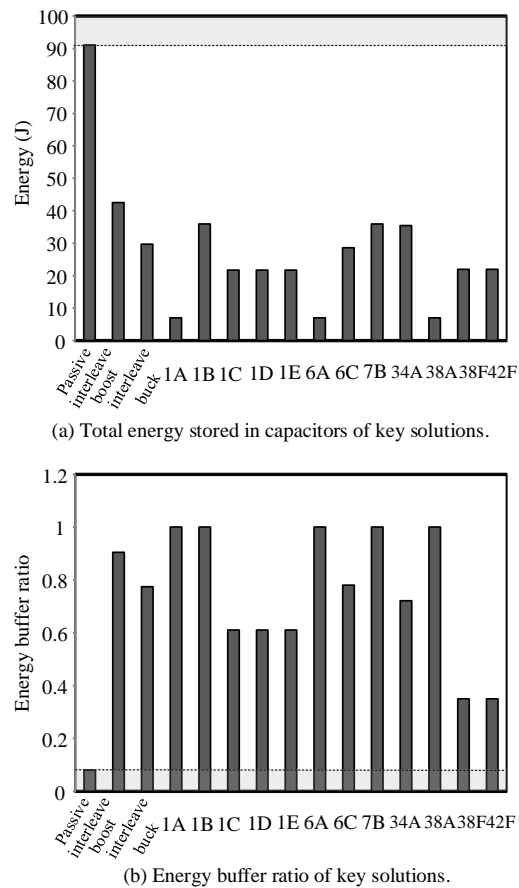
Fig. 22. Total energy stored in capacitors and energy buffer ratio comparisons among typical active DC-link solutions.
