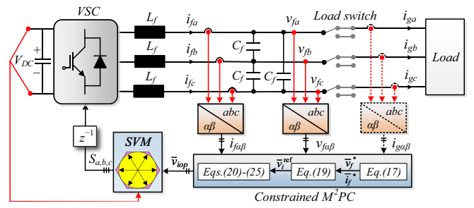
Fig. 4. Implementation of proposed constrained M 2 PC scheme for an LC-filtered VSC.
