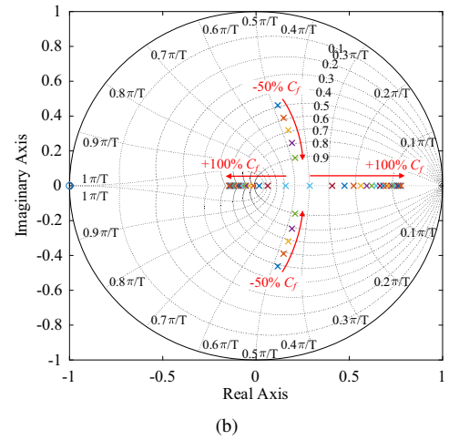
Fig. 6. Closed-loop zero-pole loci with model parameter mismatch. (a) Inductance uncertainties: -37.9\%L_f to +100\%L_f . (b) Capacitance uncertainties: -50\%C_f to +100\%C_f .
