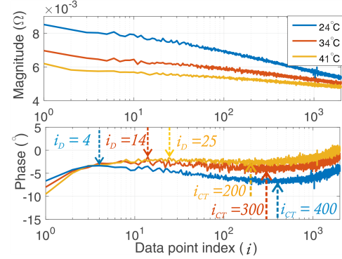
Fig. 9: Bode plot representation of the unfiltered impedance data obtained with ternary-sequence at 50% of SOC. Colored markings i_D represents the end of the diffusion part indices and i_{CT} the top of the semi-circle indices of the impedance at the corresponding temperature
