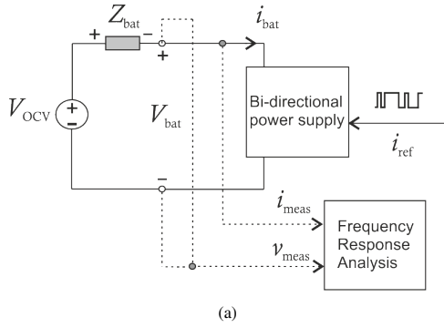
Fig. 6: a) Measurement setup configuration for the experiments b) Laboratory setup
