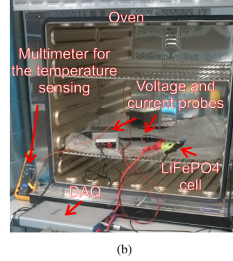
Fig. 6: a) Measurement setup configuration for the experiments b) Laboratory setup
