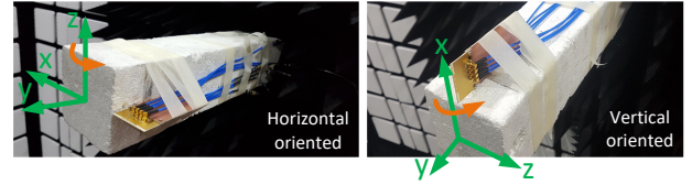
Fig. 7: The setup in the radiation pattern measurements.
