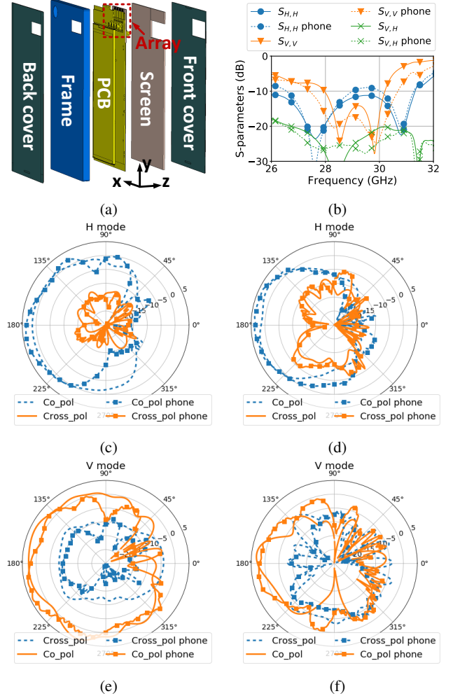
Fig. 11: The simulations of the proposed array in a mobile phone model at 28 GHz. (a) The array in the phone. (b) S-parameters of element 2 in the phone. (c) Radiation pattern of H-pol in the vertical plane (yoz). (d) Radiation pattern of H-pol in the horizontal plane (xoy). (e) Radiation pattern of V-pol in the vertical plane (yoz). (f) Radiation pattern of V-pol in the horizontal plane (xoy).
