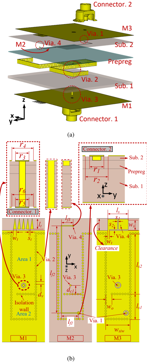
Fig. 1: Antenna configuration. (a) Exploded view. (b) Dimensions on layers.
