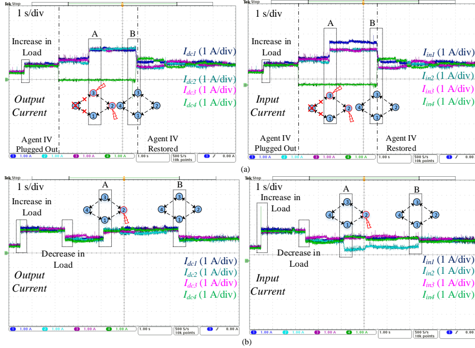
Fig. 13. Experimental validation of the proposed DE based detection theory with input and output currents: (a) Deception attack ( \mathbf{IA} = 3 ) on agent II and III when agent IV is plugged in-and-out, and (b) Deception attack ( \mathbf{IA} = 2 ) on agent II under a maximum communication delay of 65 ms. Positive DE_I for the attacked agents [calculated using (22)] ensures the presence of attack element in the corresponding agents from event A-B.
