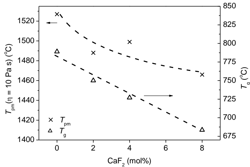
Figure A.2: Practical melting temperature ( T_{pm} ) and glass transition temperature ( T_g ) as a function of the CaF 2 content of the glasses. The dashed lines should be regarded as guides for the eye.
