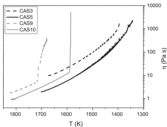
Fig. 7. Viscosity ( \eta ) change during continuous cooling of the melts in the low viscosity range. CAS3, -5 and -10 are cooled with 2 \text{ K/min} and CAS9 is cooled with 1 \text{ K/min} .
