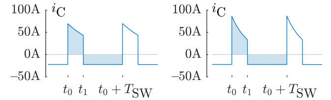
Fig. 11: Qualitative impact of zero state resistances ( R_{0H} and R_{0L} ) values on cell capacitor current on a T_{SW} time scale. Resistances halved on the right plot compared to the left plot.
