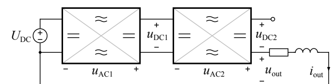
Fig. 18: Proof of concept demonstrator comprised of two daisy-chained converter cells and experimental topology.
