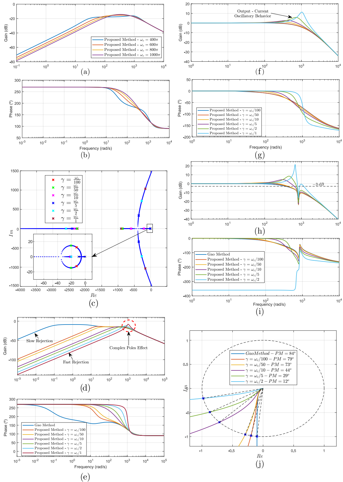
Figure 12. (a,b) Bode plot of the transfer function \left. \frac{V_c(s)}{I_o(s)} \right|_{V_c^*(s)=0} using \gamma = \frac{\omega_c}{10} ; (c) root locus of the transfer function \left. \frac{V_c(s)}{I_o(s)} \right|_{V_c^*(s)=0} ; (d,e) Bode plot of the transfer function \left. \frac{V_c(s)}{I_o(s)} \right|_{V_c^*(s)=0} ; (f,g) Bode plot of the transfer function \left. \frac{I_{LL}(s)}{I_o(s)} \right|_{V_c^*(s)=0} , (h,i) Bode plot of the transfer function \left. \frac{V_c(s)}{V_c^*(s)} \right|_{I_o(s)=0} and (j) Nyquist plot of the transfer function \left. \frac{V_c(s)}{V_c^*(s)} \right|_{I_o(s)=0} .
