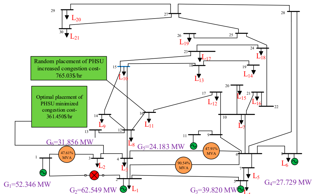
Figure 13. FPA-based cost comparison in placement of PSHU for managing congestion.
