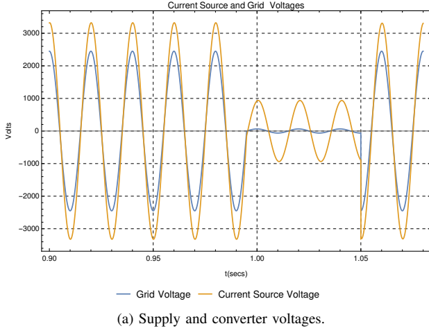
Fig. 3: Ideal test results
