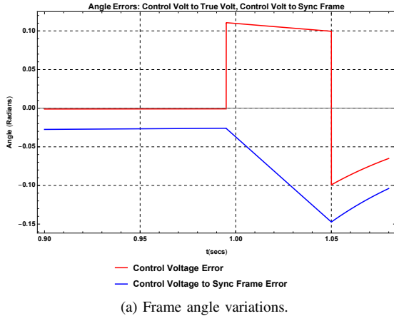
Fig. 4: Ideal simulation results for i_d = 0\text{kA} and i_q = -46.67\text{kA} (i.e. -90^\circ ), Dip \hat{V}_G = 0.0258\text{pu} .
