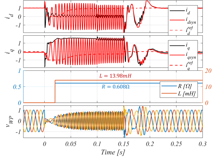
(b) Identification of grid impedance during current injection based on the grid code. \hat{R} = 0.608\Omega and \hat{L} = 13.98mH .
