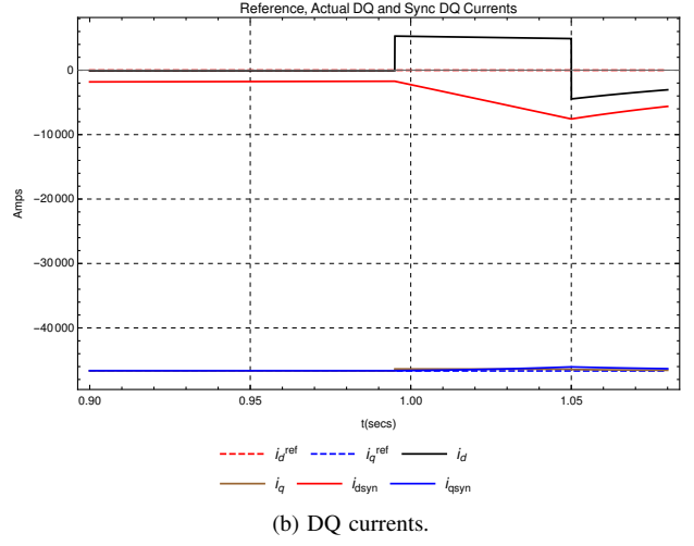
Fig. 3: Ideal test results
