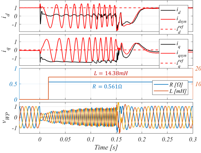
(a) Identification of grid impedance during active current injection. \hat{R} = 0.561\Omega and \hat{L} = 14.38mH .
