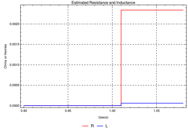
Fig. 4: Ideal simulation results for i_d = 0\text{kA} and i_q = -46.67\text{kA} (i.e. -90^\circ ), Dip \hat{V}_G = 0.0258\text{pu} .
