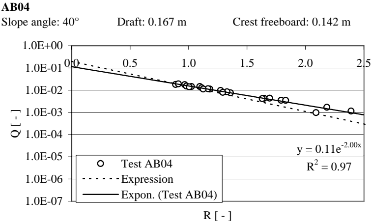
Figure B.9: Results of tests with test geometry AB04.
