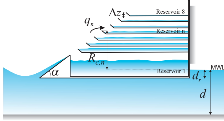
Figure 4.2: Geometric parameters used for multi level reservoirs.
