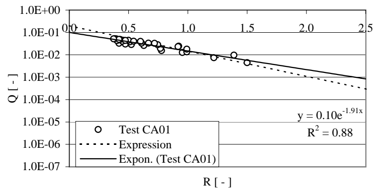
Figure B.22: Results of tests with test geometry CA01.
