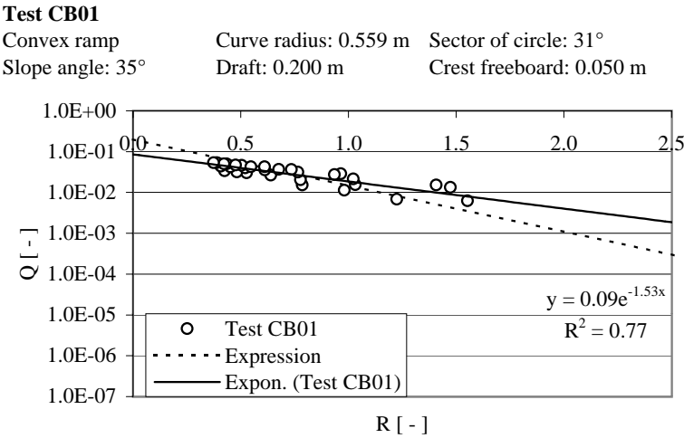
Figure B.28: Results of tests with test geometry CB01.
