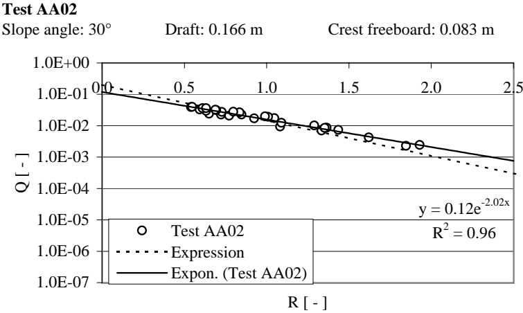
Figure B.2: Results of tests with test geometry AA02.
