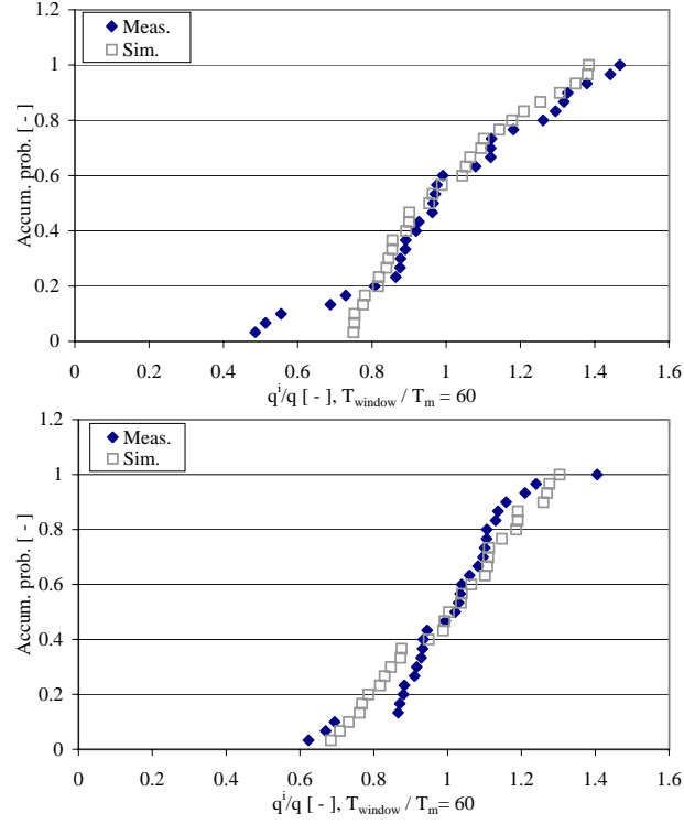
Figure 3.24: Results for the two tests with R = 0.61 (top) and 0.37 (bottom). The accumulated probability density for \frac{q_{\text{window}}^i}{q} is plotted for q_{\text{meas}}(t) and q_{\text{sim}}(t) , respectively.
