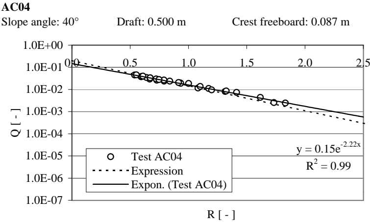
Figure B.13: Results of tests with test geometry AC04.
