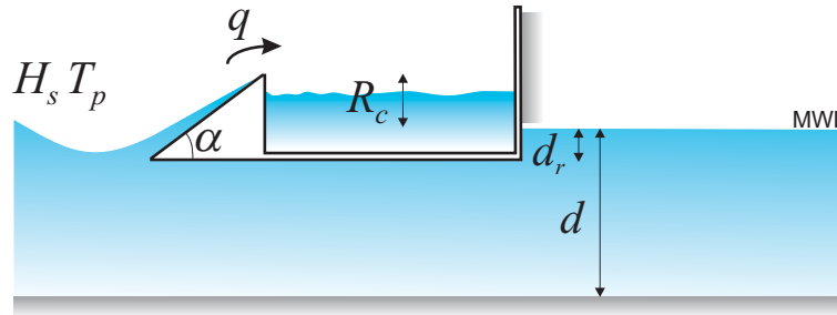
Figure 3.2: Geometric parameters used for linear slopes.
