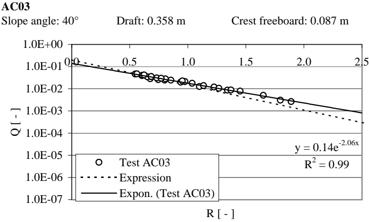
Figure B.12: Results of tests with test geometry AC03.
