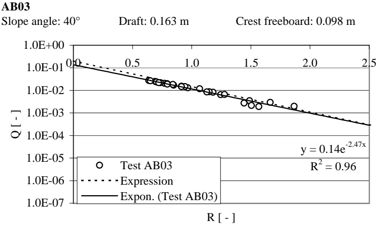
Figure B.8: Results of tests with test geometry AB03.
