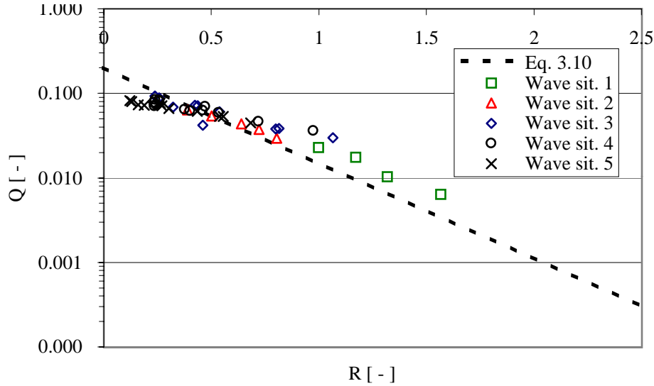
Figure 4.23: Non-dimensionalized total overtopping discharge (sum of all reservoirs) as a function of dimensionless freeboard, compared with eq. 3.10.
