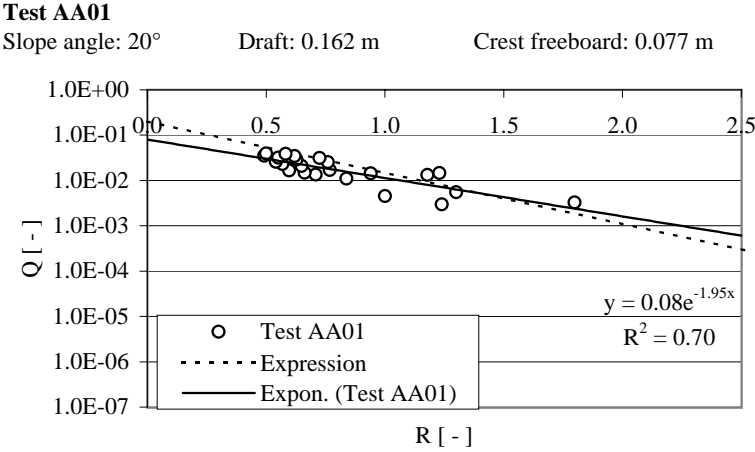
Figure B.1: Results of tests with test geometry AA01.
