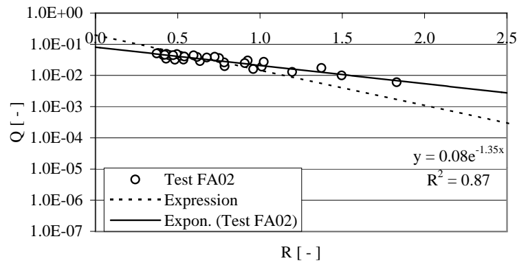
Figure B.39: Results of tests with test geometry FA02.
