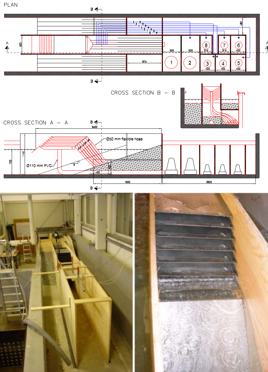
Figure 4.5: Drawings and photos of the model test setup as constructed in the wave flume. Top: Plan view. Middle: Cross section A - A and B - B. Measures are in mm (model scale). Bottom, left: Model test setup before the flume is filled with water. Bottom, right: The model in action.
