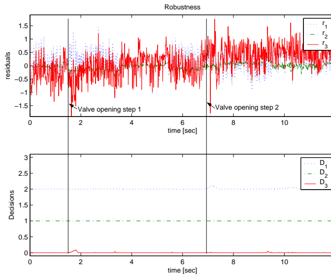
(a) Robustness test.
