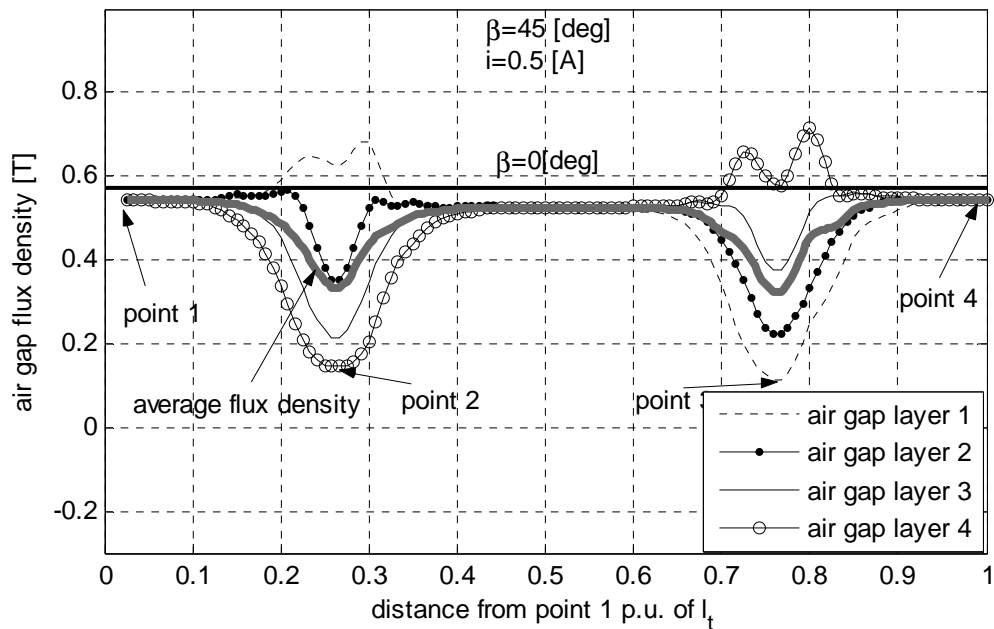
Fig.B.12 Flux density distribution in the four layers of the air gap in a Shark SRM ( \beta=45[\text{deg}] ), at low current
