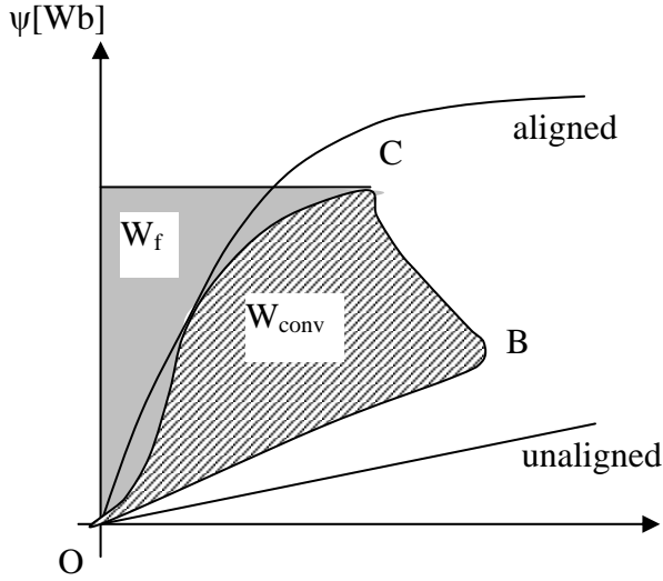
Fig. 1.9 Conversion loops for the SRM illustrating the main points used in controlling the SRM
