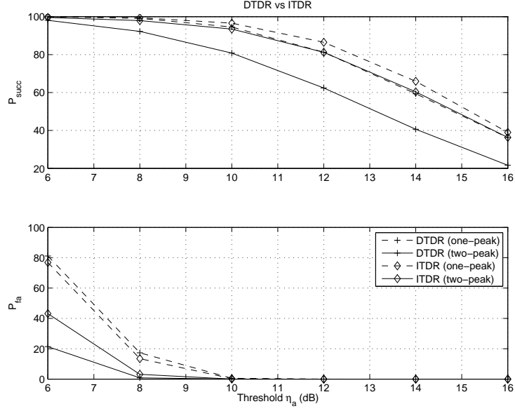
Figure 3.9: Success and false alarm probabilities for DTDR and ITDR schemes as function of the detection threshold
