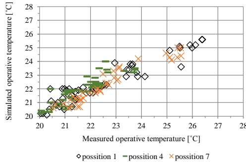
Figure 13: Comparison of simulated T_{\text{op}}^S with the new zone model in IDA ICE and measured T_{\text{op}}^S for position 1, 4 and 7. Total observations n=147 , correlation coefficient R=0.95 (position 1), R=0.89 (position 4) and R=0.96 (position 7).
