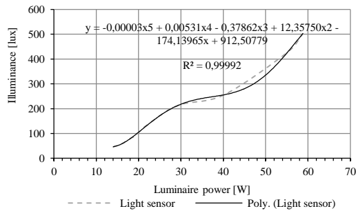
Figure 9: Dimming characteristics of the luminaire in the Cube.
