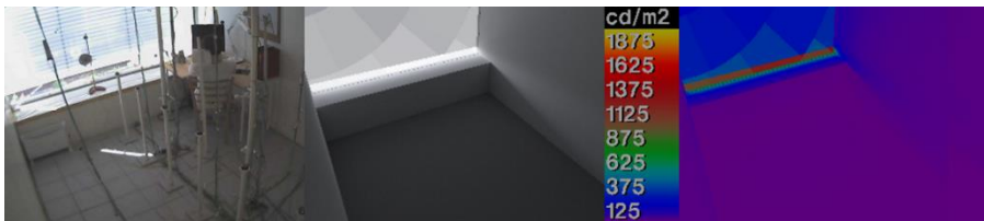
Figure 18: Photo of the experiment room at 09.30, 23.07.2014 and rendering from Radiance showing that the light stripe penetrating into the room is not detected in the simulation.
