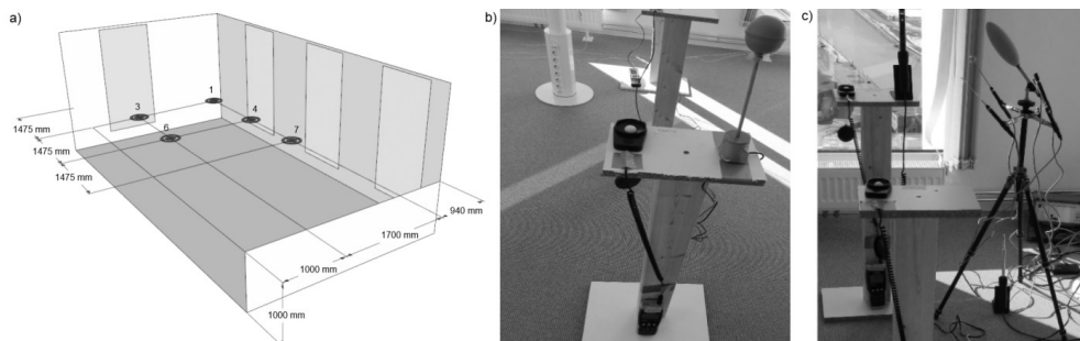
Figure 2: a) Illustration of the placement of the globe thermometers for measurements of operative temperature. b) and c) Photo of the measurement setup; globe thermometer (b) and the Innova Thermal Comfort Data logger (c) (photo: Silje Bjørkeng).
