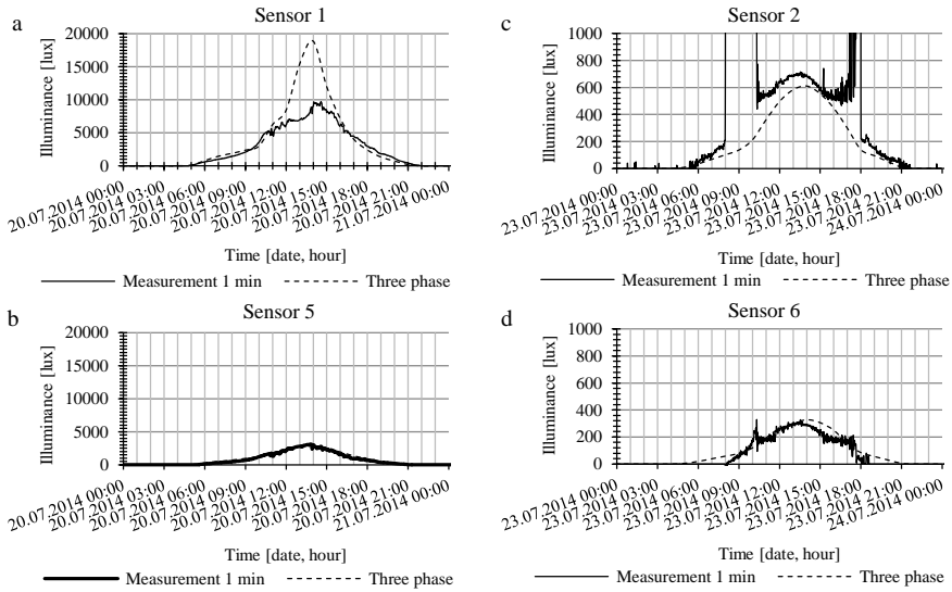
Figure 16: Comparison measurements and simulations in the experimental room in Aalborg for a sunny day without shading (a-b) and a sunny day with activated solar shading (c-d).
