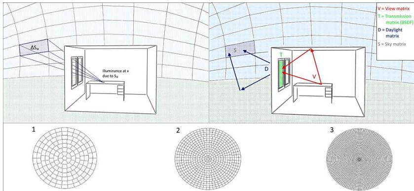
Figure 4: Principle illustration of the Daysim method (left, after [96]) and the three-phase method (right, after [152]) and the sky patch sub division according to (1) modified Tregenza-145, (2) Reinhart -581 and (3) Reinhart -2321.
