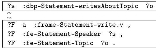
Fig. D.3: The general pattern of a dereification rule.
