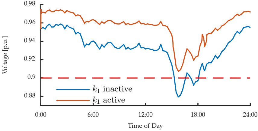
Fig. E.1: Voltage magnitude at bus B_3 in Figure E.6, with and without the local voltage controller k_1 active. Lower voltage bound is given by the red dashed line.
