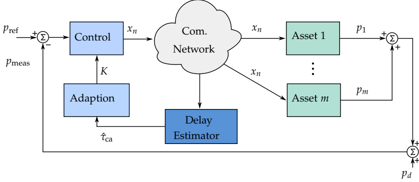
Fig. 3.8: Control system architecture. Controller gains, (K_{p,i}, T_{l,1}) , are adapted based on estimates of the communication network state, \hat{S}_i .
