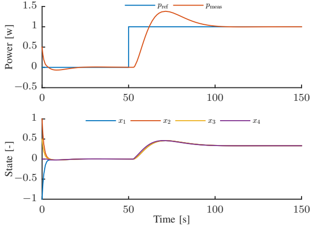
Fig. B.14: Step response of system with a congested communication network and \tau_{ca} = 2.85 s. The control parameters are, K_P = -0.04 , T_I = 20 Top: reference tracking. Bottom: agent state values. Notice that leader-follower consensus is achieved when the reference value is reached.
