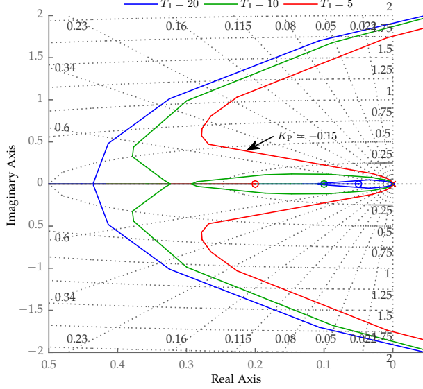
Fig. B.11: Root-locus plot of the controlled system, with a non-congested communication network. The root-locus is plotted for three different integral time values and the arrow indicates the choice of gain value. The graph has been zoomed in to show the critical part of the locus.
