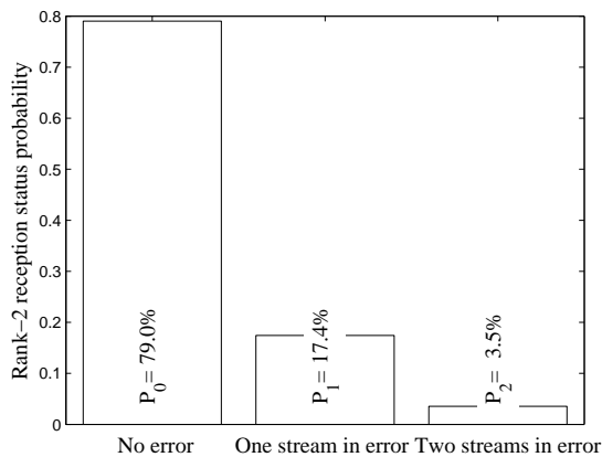
Fig. 5.15: Reception error probabilities for rank-2 transmissions. Full buffer model is used with 10 users per cell.
