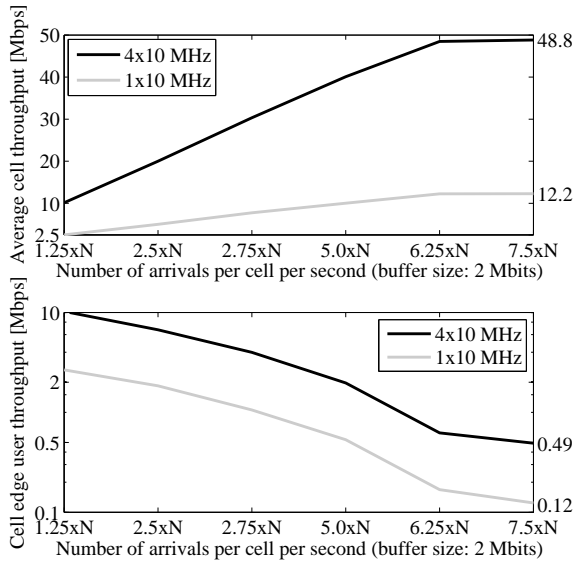
Fig. C.5: Performance comparison: single-CC versus 4-CC.
