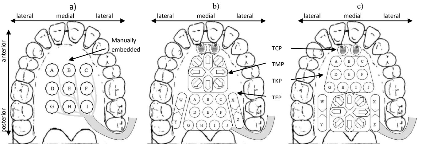
Figure 2-2. Superior view of keyboard/joystick layout options; a) L_0 – Palatal plate with 9 inductive coils. b) L_1 – PCB palatal plate where the Tongue Mousepad (TMP) is located in the anterior part of the hard palate and the Tongue Keypad (TKP) in the posterior part. c) L_2 – PCB palatal plate where the TKP is located in the anterior part of the hard palate and the TMP in the posterior part. L_0 has only 9 key-sensors, while L_1 and L_2 have a TMP with 8 mouse-sensors, a TKP with 10 key-sensors, 2 left/right click sensors, and 4 extra key-sensors (oval). (Caltenco Arciniega et al. 2011)
