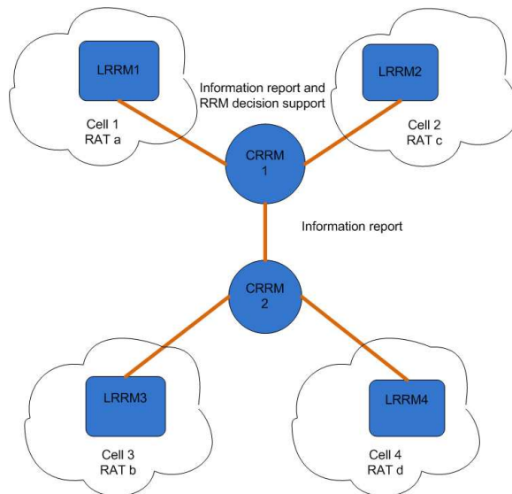
Figure 3.1: 3GPP CRRM functional model
