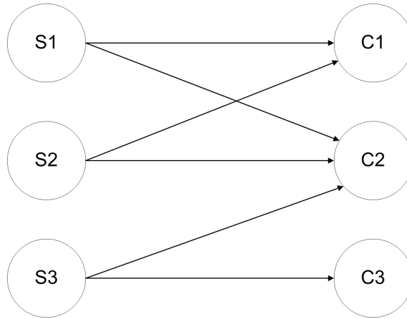
Figure 8.2: Correlation graph
