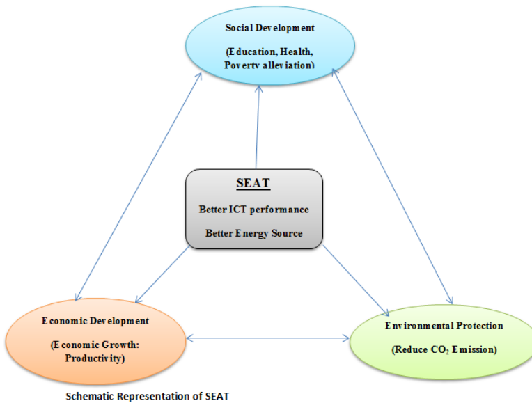
Figure 8. 6 SEAT Framework.
