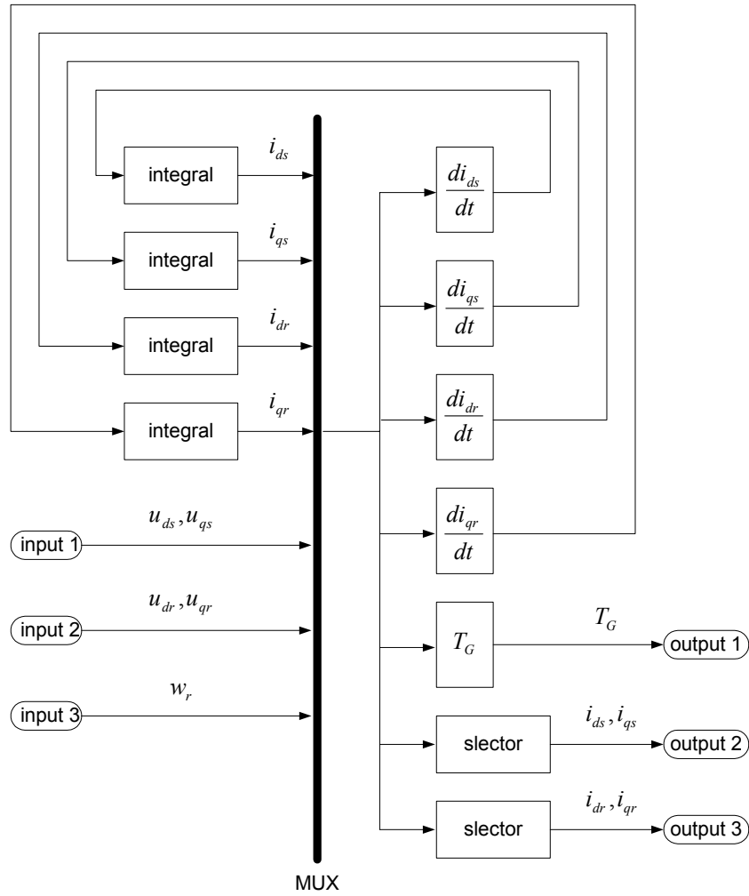
Figure 2.12 Block diagram of the DFIG model.
