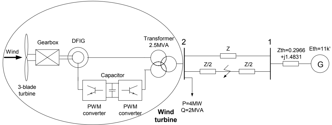
Figure 7.1 Diagram of the simulated system with wind turbine and grid.
