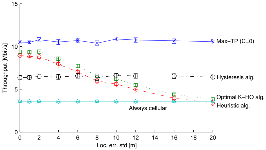
Figure 7.14: Performance impact of increasing localization error.
