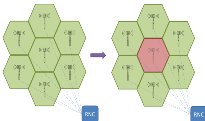
Figure 7.2 – Graphical representation for site sleep mode. A centralized RNC monitors the load of various sites and based on preset conditions gradually execute sleep mode for selected sites.
