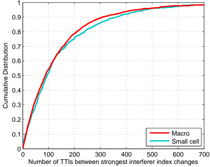
Fig. 12: Cumulative distribution function of the number of TTIs between changes in strongest interferer index.
