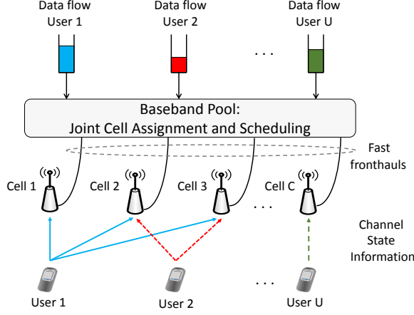
Fig. 2: System model
