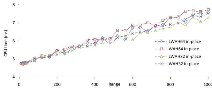
(b) Total CPU Time using UCOR on the Music Attributes
