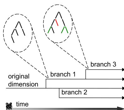
Figure 2.9: Versioned Hierarchies
