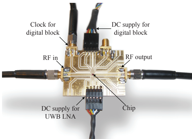
Figure 3.5: The PCB with the bonded chip for the measurements.
