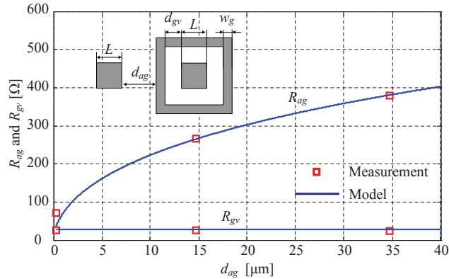
Figure 5.26: Measured and calculated aggressor-to-guard ring and guard ring-to-victim resistance versus aggressor-to-guard ring distance. The parameters used in this case are: L = 20 \mu\text{m} , d_{gv} = 0.28 \mu\text{m} , and w_g = 5 \mu\text{m} .
