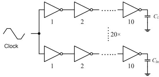
Figure 4.11: The schematic of the inverter chain block for the simulation of switching noise.
