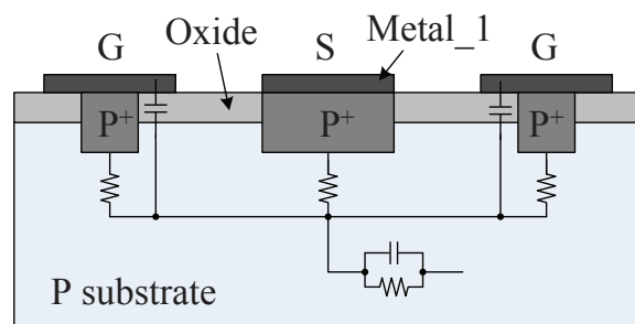
Figure 2.8: The cross section view of the improved substrate noise measurement fixture.
