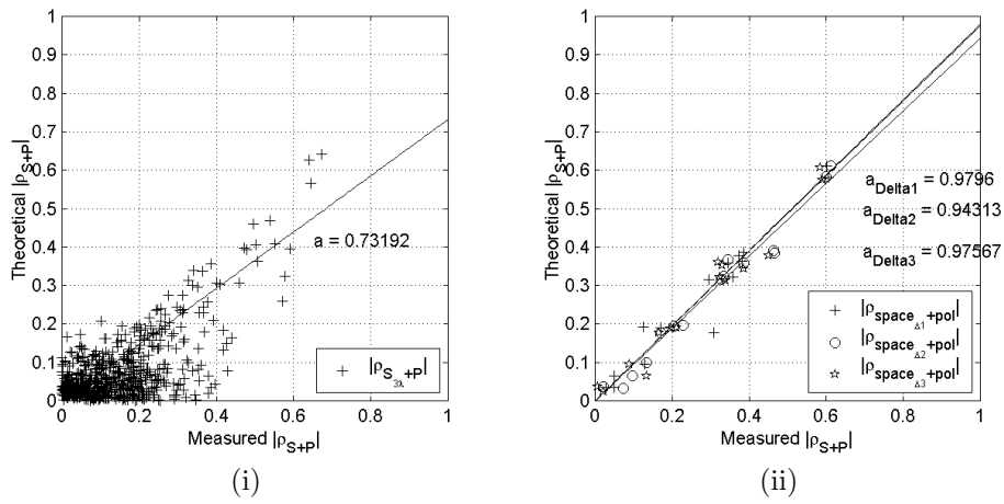
Figure G.3: Scatter diagram of the measured |\rho_{spatial+pol}| versus the theoretical |\rho_{spatial+pol}| for measurement using a \pm 45^\circ antenna patch in (i) picocell (METRA) and (ii) microcell (SUNBEAM).
