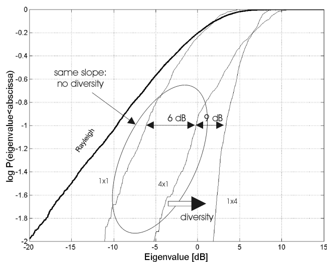
Figure 2.5: Empirical illustration of the antenna gain and the diversity gain for different spatial antenna array configuration set-ups for the correlated scenario. AS-BS:low -MS:high.
