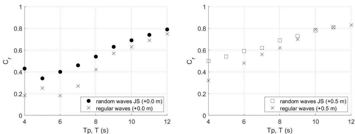
Fig. 5. Comparison between the reflection coefficient calculated using random waves with JONSWAP spectra ( H_{m0}=1.5 m) and regular waves ( H=1.5 m) for the 4-rows perforated caisson. For both cases the wave height is 1.5 m. Left: reference water level. Right: +0.5 m water level.
