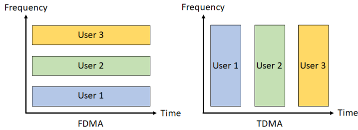
Figure 1.15 FDMA and TDMA techniques.
