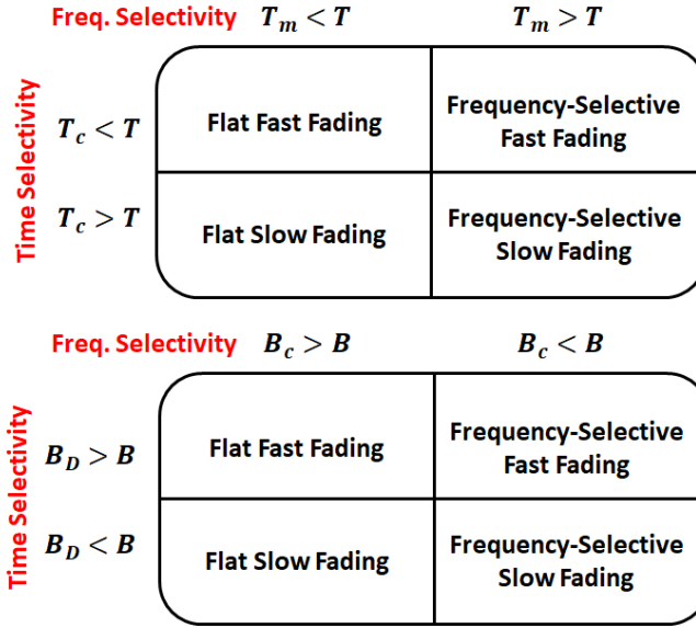
Figure 1.13 Classification of fading channels.
