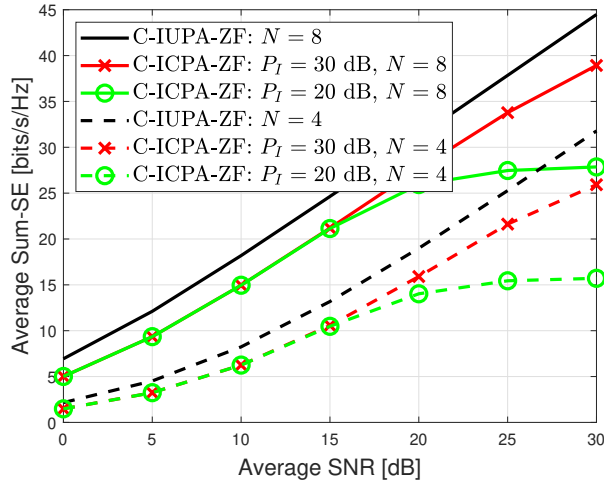
(a) C-ICPA-ZF for N = 4 and N = 8 .
