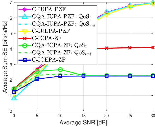
(a) C-IUPA-PZF vs. C-ICPA-ZF variants for P_l = 5 dB and P = 0 dB.
