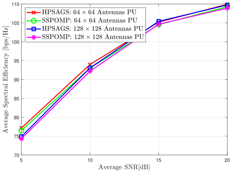
Figure 5.6 128 × 128 secondary link, 64 × 64 and 128 × 128 primary link.
