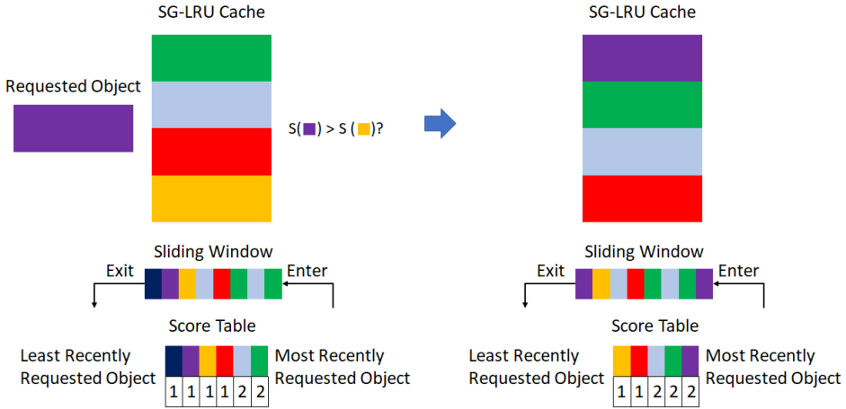
Figure 3.1 Replacement operation of an SG-LRU cache with size C = 4 that utilizes the WLFU score function with a sliding window of size W = 8 .
