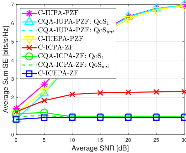
(b) C-IUPA-PZF vs. C-ICPA-ZF variants for P_l = 0 dB and P = 0 dB.
