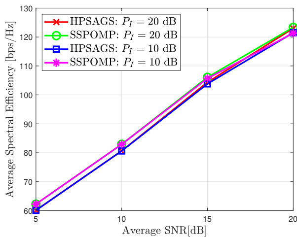
Figure 5.4 ICPA for U-SVD, HPSAGS, and SSPOMP with varying IPT.
