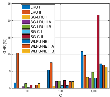
(b) Global hit rates.
