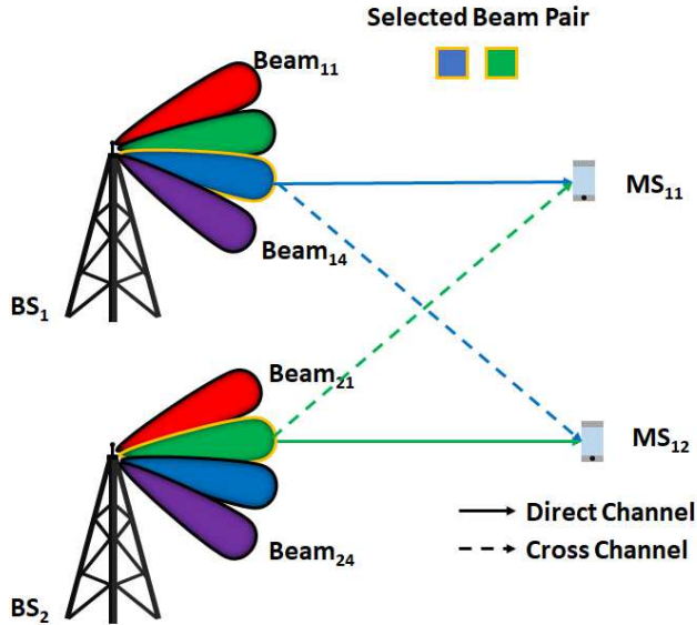
Figure 4.4 Beam selection.
