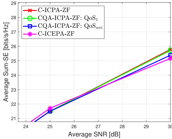
(b) C-ICPA-ZF vs. CQA-ICPA-ZF vs. C-ICEPA-ZF with P_I = 30 dB and P = 0 dB.
