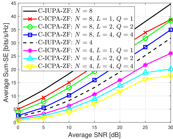
(b) C-ICPA-ZF for a SISO and various MIMO PS setups and varying number of BS antennas with P_I = 30 dB and P = 0 dB.
