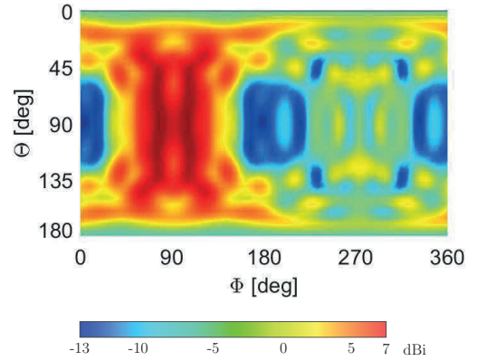
Fig. 8. Total Scan Pattern (TSP) of the lens antenna placed in the corner of the PCB mobile phone simulated at 38 GHz.
