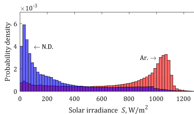
Figure 10. Density distribution of the solar irradiances.
