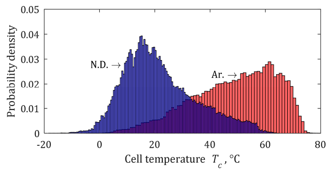
Figure 12. Density distribution of the cell temperatures.
