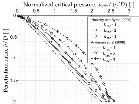
Fig. 2.3: Normalized critical pressure versus penetration ratio with the k_{\text{fac}} influence (Houlsby and Byrne, 2005; Andersen et al., 2008)
