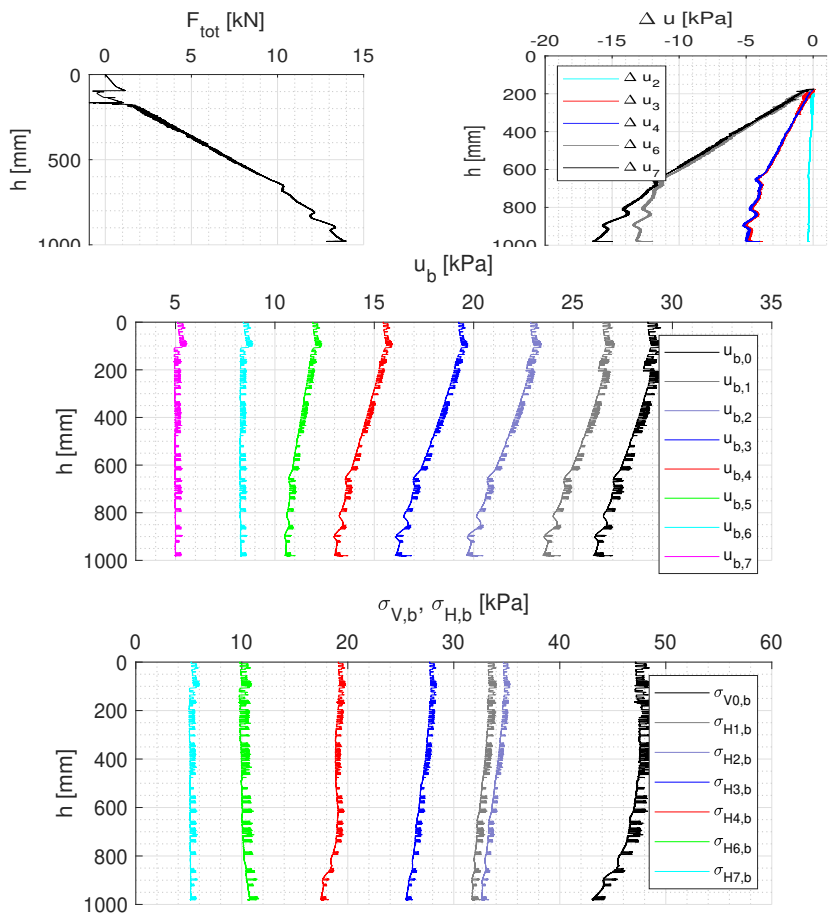
Fig. F.43: Results of installation test
