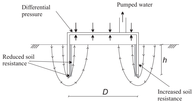
Fig. 1.9: Seepage around the skirt during suction installation in sand (Koterás et al., 2016)
