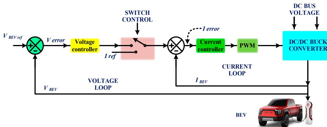
Figure 6. Charging and discharging of a BEV battery.
