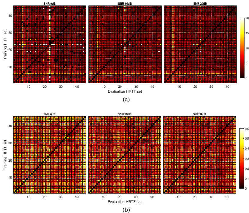
Figure 2. Speech-in-noise localization predictions resulting from auditory model simulations on 45 CIPIC subjects in the horizontal plane with three different SNRs. “All-against-all” matrices for (a) horizontal error [deg], and (b) front-back confusion rate [%]. White cells in the matrix (when present) denote values higher than the full-scale.
