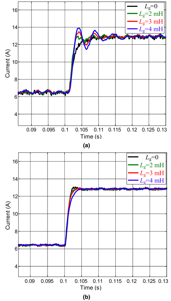
FIGURE 8. The transient performances when the grid inductance varies from 0 mH to 4 mH under the different control strategies. (a) PI + DOB. (b) APID + DOB.
