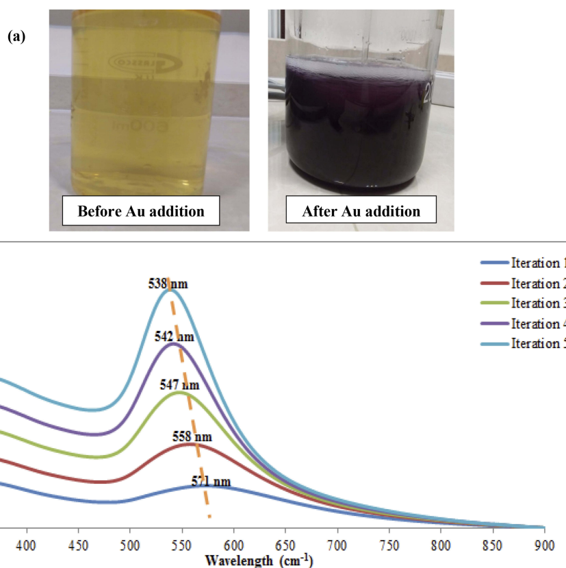
Figure 2 (A) Changing the solution color before and after of Au addition, (B) UV-Visible spectroscopy of five Au iterations.
