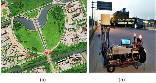
Fig. 1. (a) Measurement environment. (b) Setup used at Rx side.
