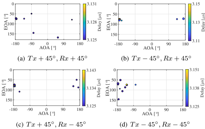
Fig. 10. PADP at arrival side (DOA).
