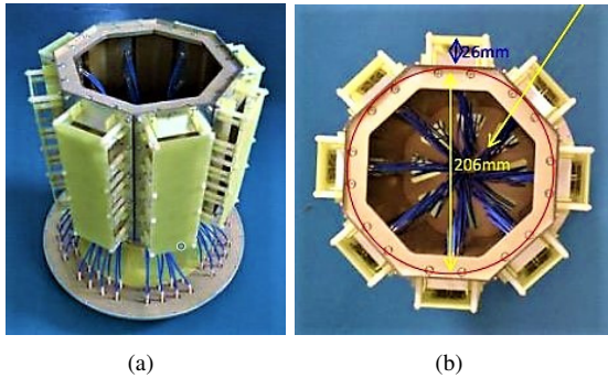
Fig. 3. Rx antenna array: (a) Side view; (b) Top view.
