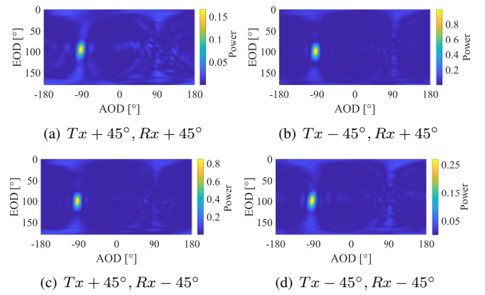
Fig. 4. PAS at departure side (DOD).
