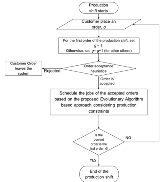
FIGURE 1. A framework for multiple order PFSPs.
