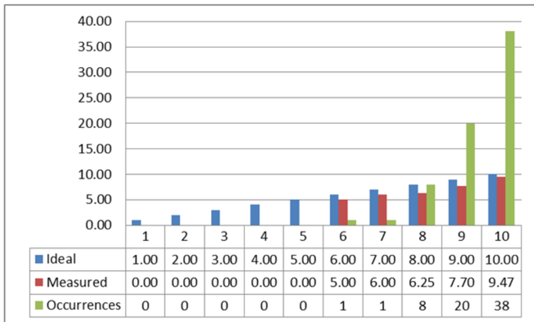
Figure 6: Phrase types
