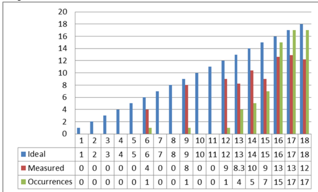
Figure 4: Clause constituents
