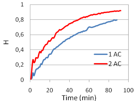
Figure 8. The air cleaner effectiveness H for one AC and two ACs
