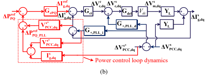
Fig. 2. Block diagram of Fig. 1(a). (a) Based on real space vectors and transfer matrices [9]. (b) Based on complex space vectors and complex transfer functions.
