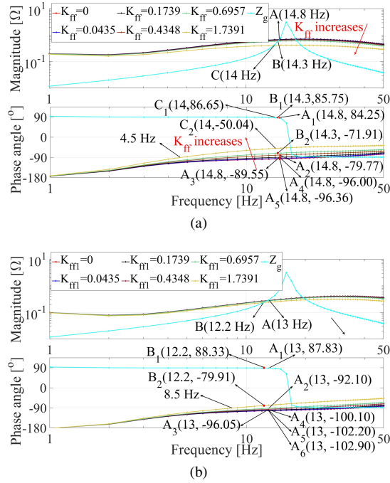
Fig. 4. Bode diagrams of q-axis impedance component. (a) Bode diagrams of Z_{qq}^{PLL} with different K_{ff} . (b) Bode diagrams of Z_{qq}^{PCL} with different K_{ff1}
