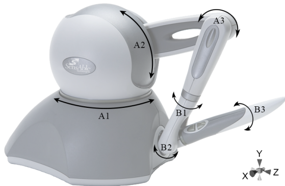
Figure 4. The PHANTOM Omni has six axes of rotation, three of which provide force feedback (A1-3), and three only tracking position (B1-3). Together, these axes provide six degrees of freedom: x , y and z positions of B2 (according to the shown coordinate system) and rotations of the pen.
